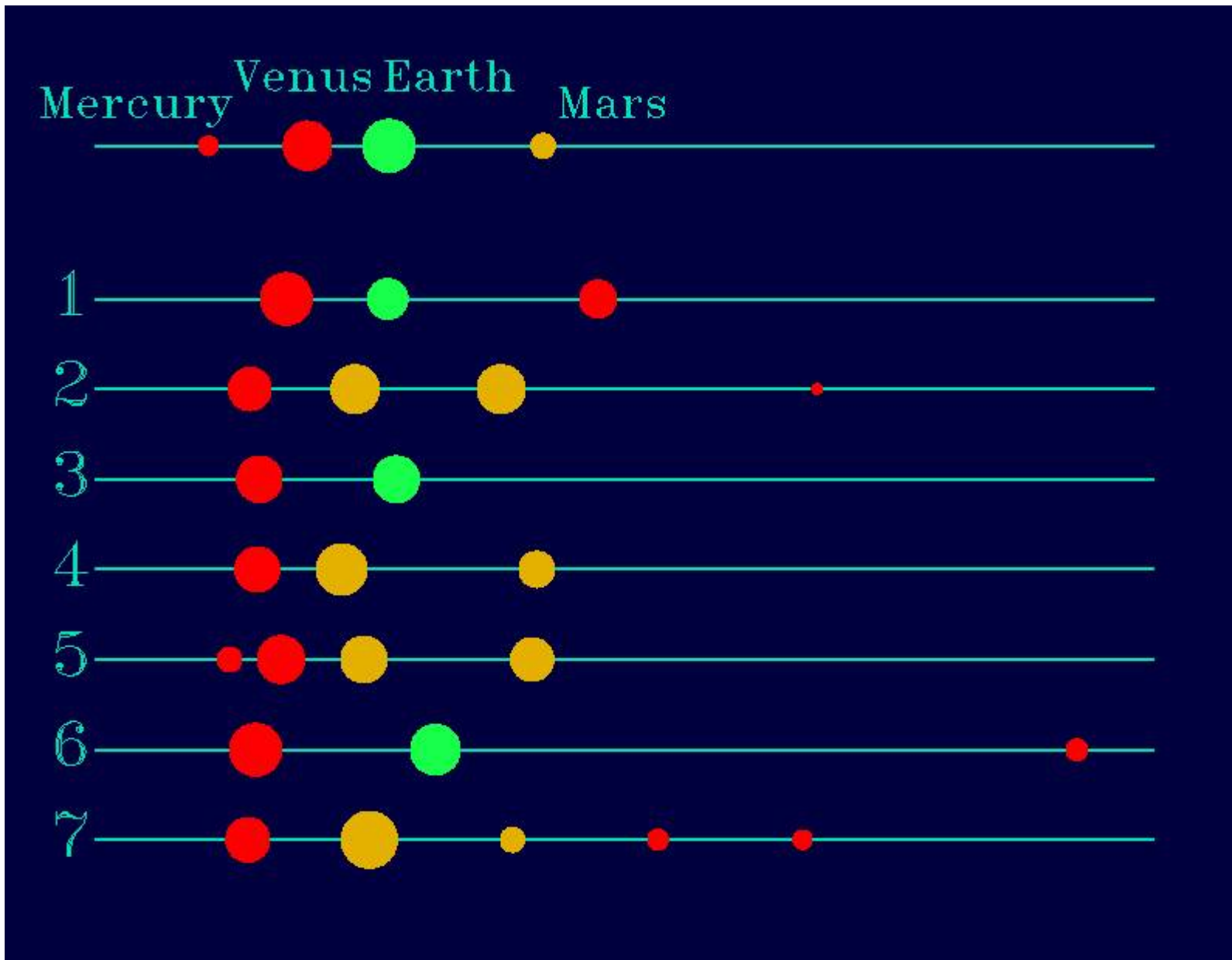
Seven planetary systems simulated on a computer
