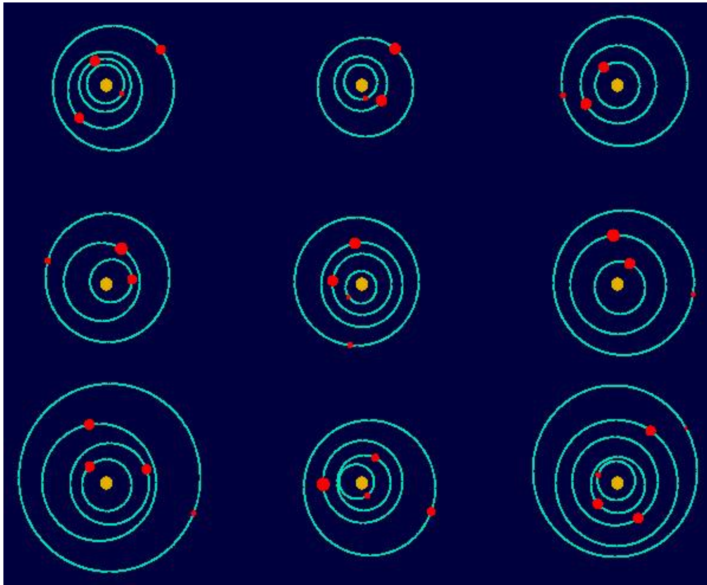
Some model planetary systems showing the terrestrial (rocky) planet orbits.
